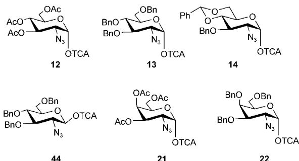
Figure 4. Glycosyl donors.
